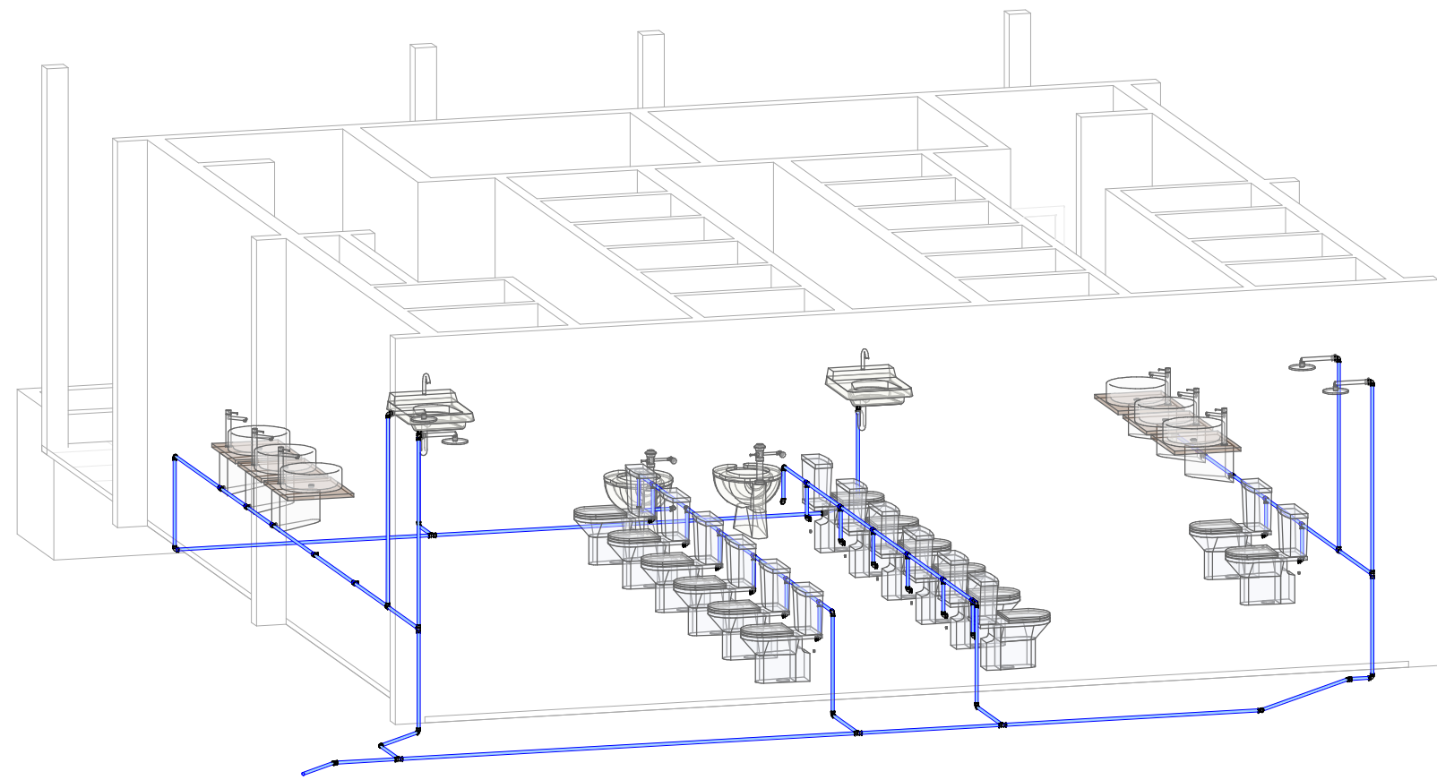
5 VISTA ABS - 3D ESCALA -
